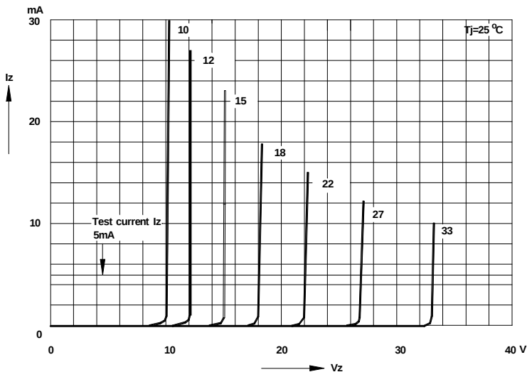
Breakdown characteristics
