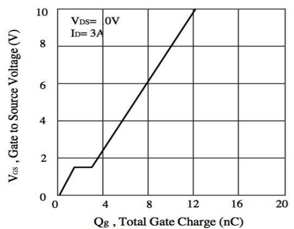
Figure 6. Gate Charge
