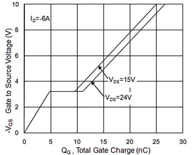
Fig.4 Gate-Charge Characteristics
