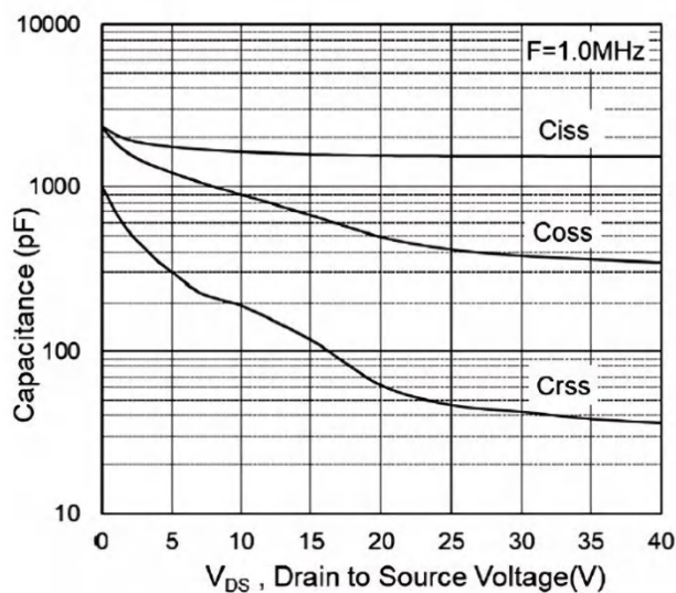
Fig.7 Capacitance
