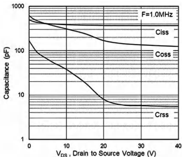
Fig.7 Capacitance
