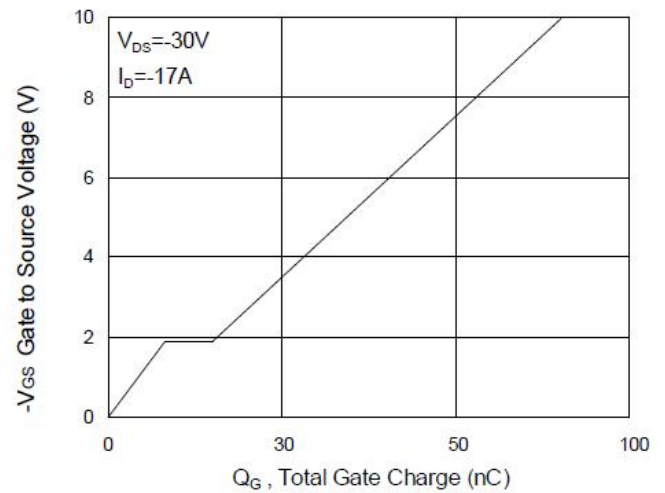
Fig.4 Gate-Charge Characteristics
