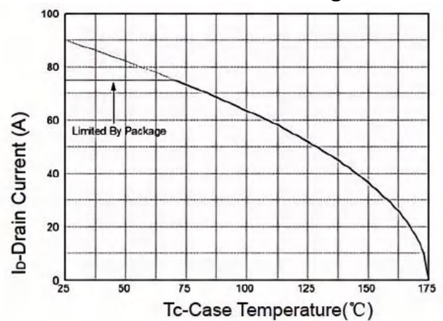
Fig.8 Drain Current
