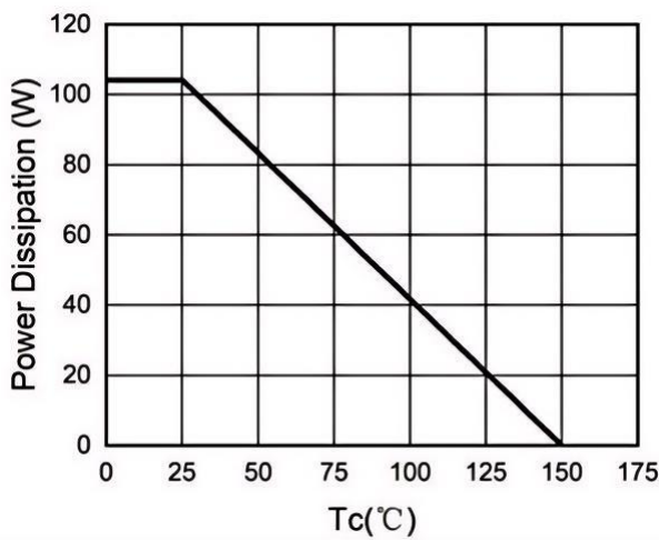
Fig.3 Power Dissipation
