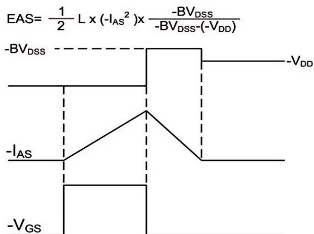
Fig.8 Unclamped Inductive Waveform
