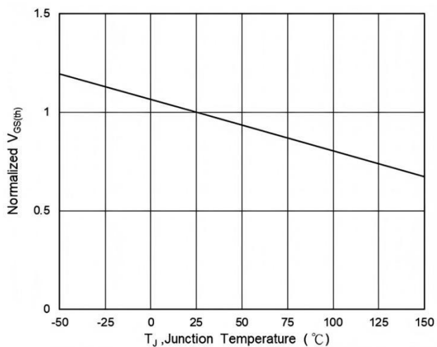
Fig.5 Normalized V_{TH} vs T_J
