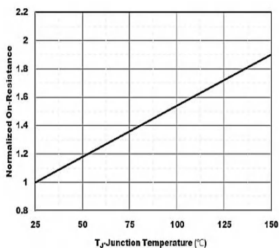
Figure6. Normalized On-Resistance
