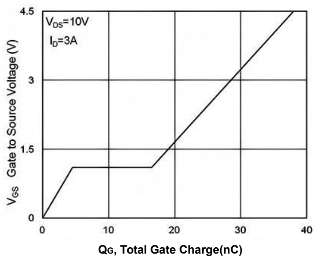
Fig.4 Gate-Charge Characteristics
