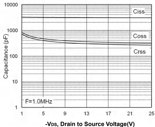
Fig.8 Capacitance
