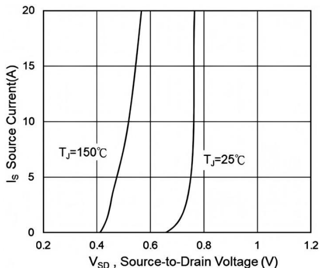
Fig.3 Source Drain Forward Characteristics
