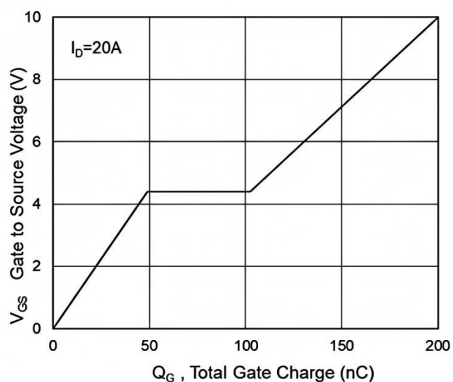
Fig.4 Gate-Charge Characteristics
