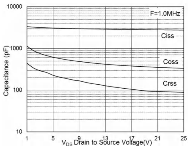
Fig.7 Capacitance
