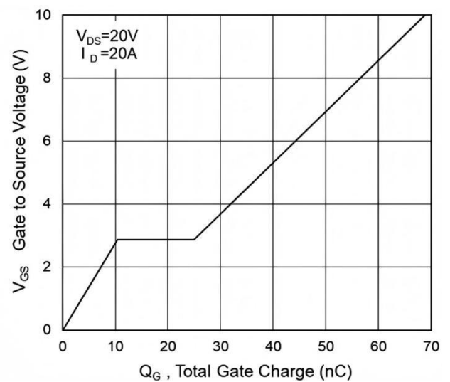
Fig.4 Gate-Charge Characteristics
