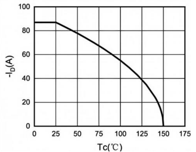
Fig.4 Drain Current
