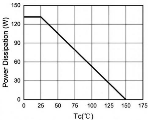
Fig.3 Power Dissipation
