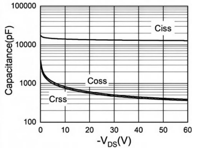
Fig.8 Capacitance
