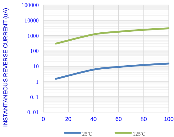
Fig.3-TYPICAL REVERSE CHARACTERISTICS
