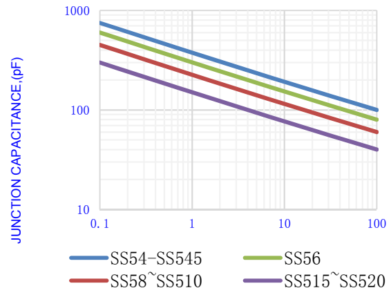
Fig.4-TYPICAL JUNCTION CAPACITANCE
