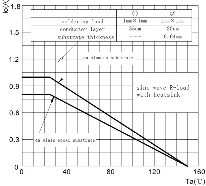
FIG1:Io-Ta Curve
