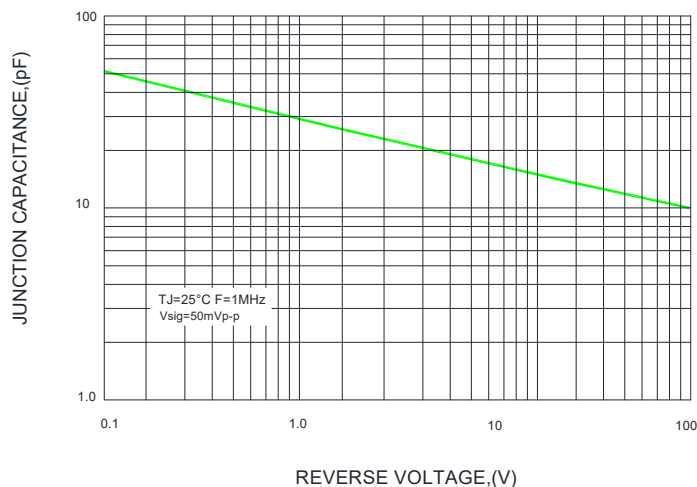
FIG.5-TYPICAL JUNCTION CAPACITANCE
