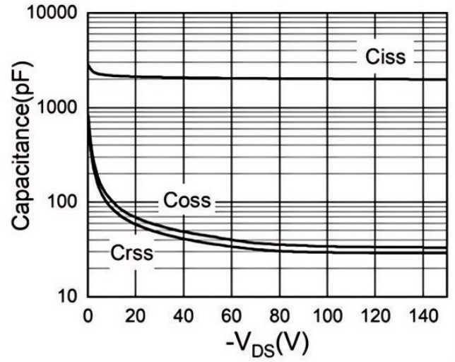
Fig.8 Capacitance
