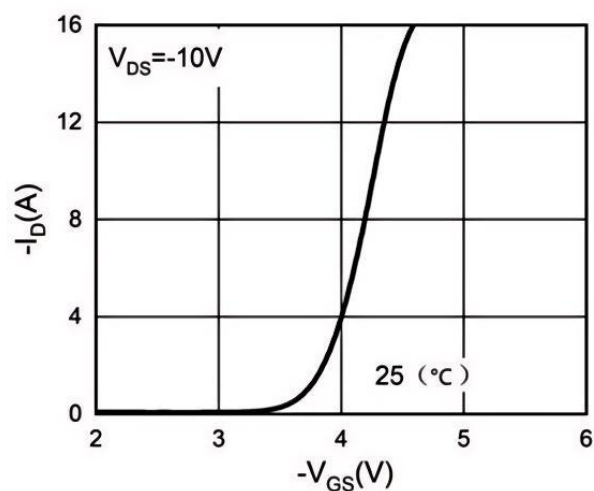
Fig.2 Transfer Characteristics
