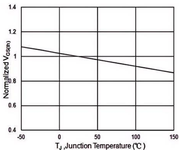
Fig.5 V_{GS(th)} vs T_J
