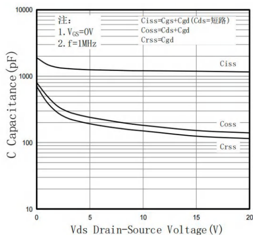
Fig.6 Capacitance Characteristic
