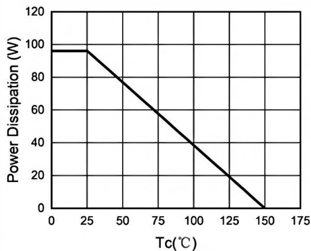
Fig.3 Power Dissipation
