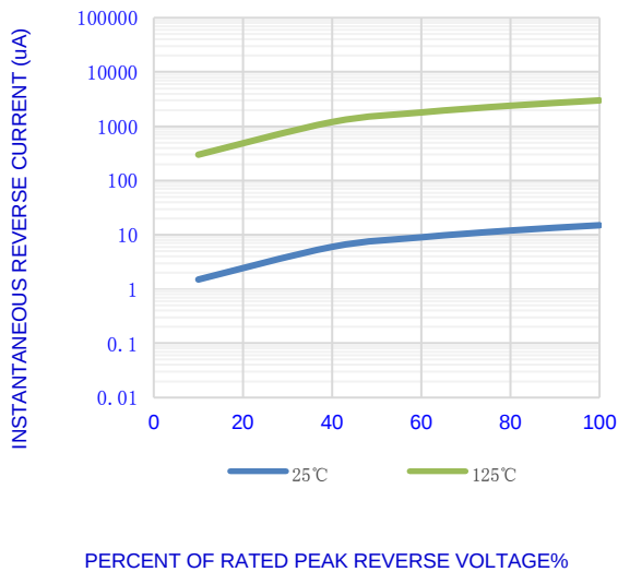
Fig.3-TYPICAL REVERSE CHARACTERISTICS
