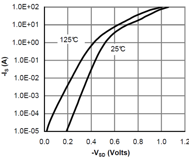
Figure 6: Body-Diode Characteristics
