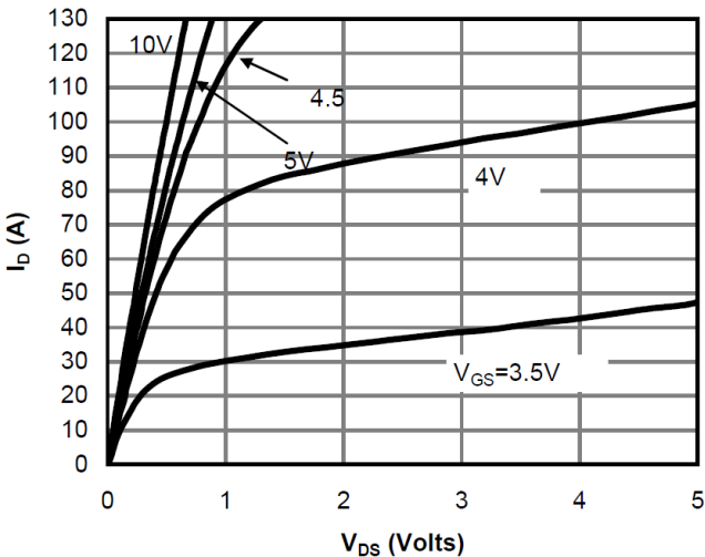
Fig 1: On-Region Characteristics
