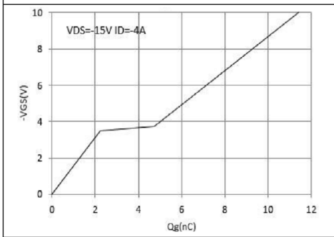
Figure 7. Gate-Charge Characteristics
