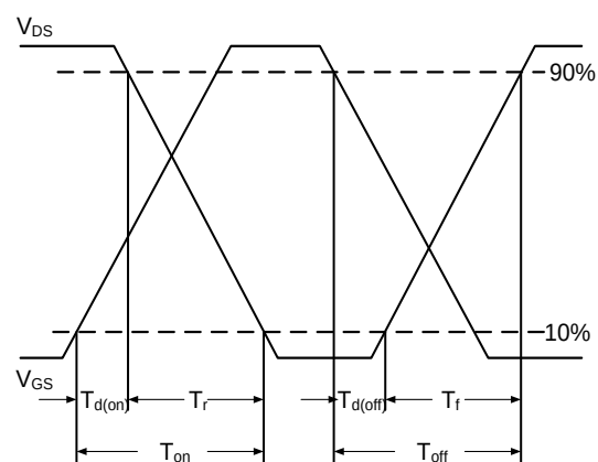
Fig.8 Switching Time Waveform
