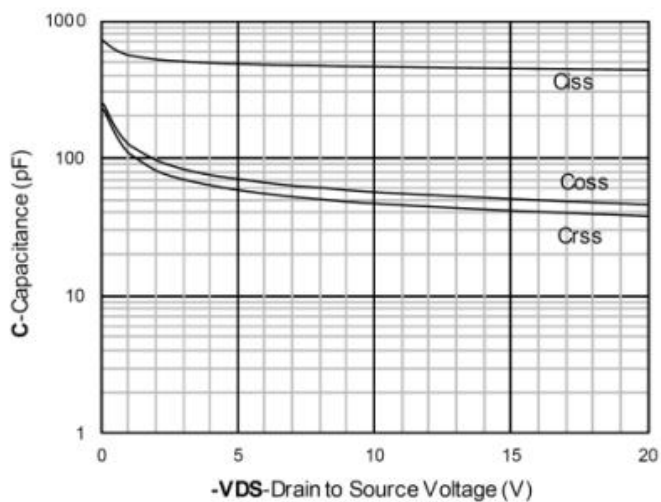
Capacitance Characteristics
