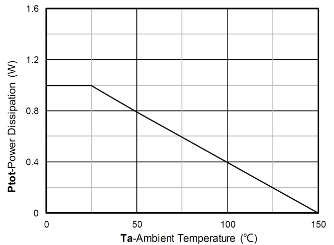
Power dissipation
