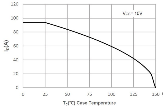
Maximum Continuous Driain Current vs. Case Temperature
