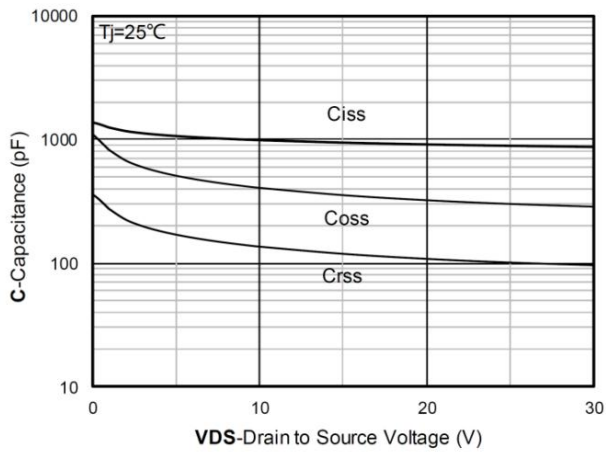
Capacitance Characteristics
