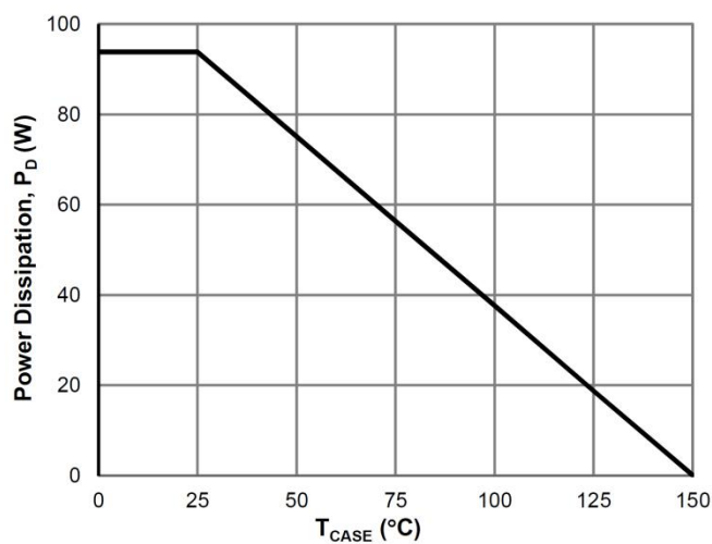
Power De-rating
