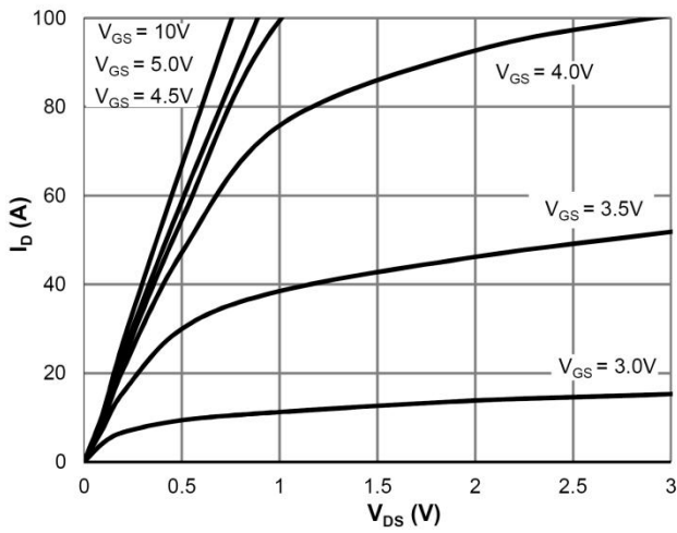
Saturation Characteristics
