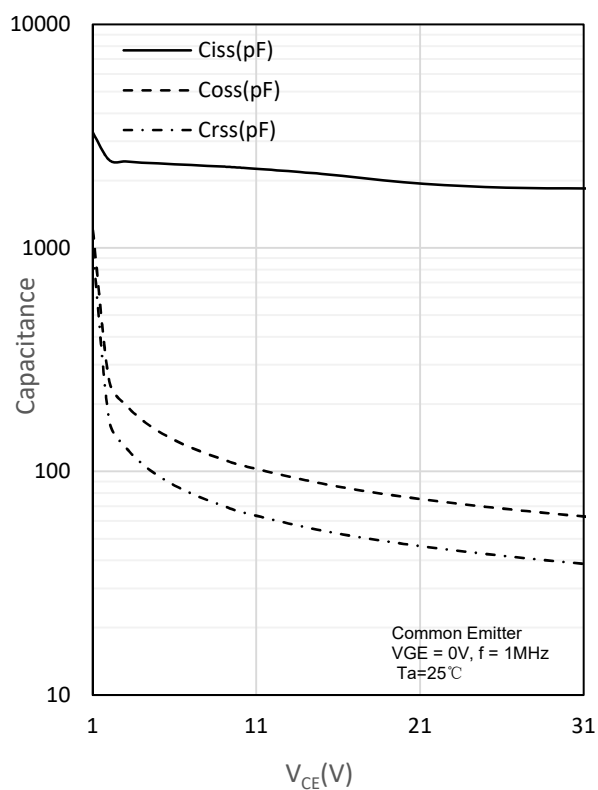
Fig. 10 Capacitance characteristics
