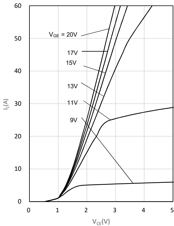
Fig. 3 Output characteristics
