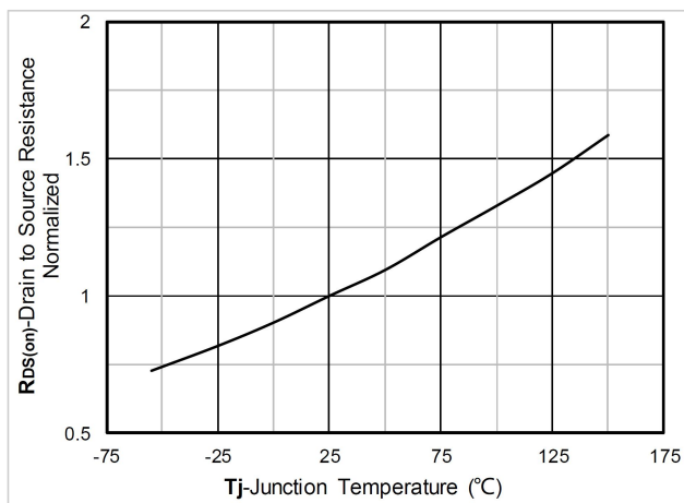
Normalized On-Resistance
