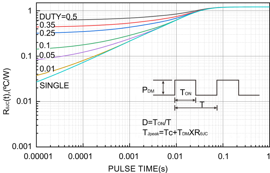
Fig9. Thermal Response
