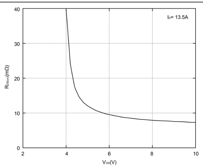
Fig2. Typical Output Characteristics
