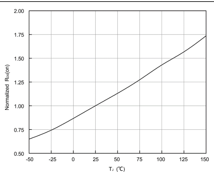
Fig6. Normalized R_{DS(on)} vs T_j
