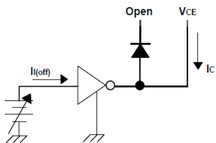
Fig.3 Iloff Test Circuit
