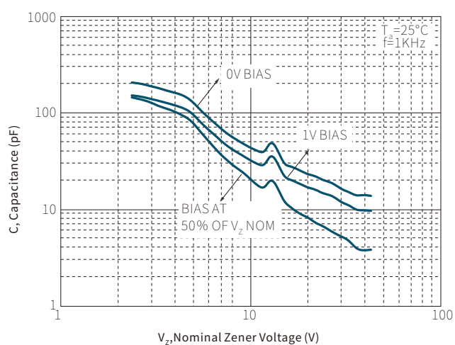
Typical Capacitance
