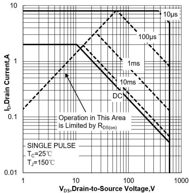
Figure 1b Safe Operating Area (FullPAK)
