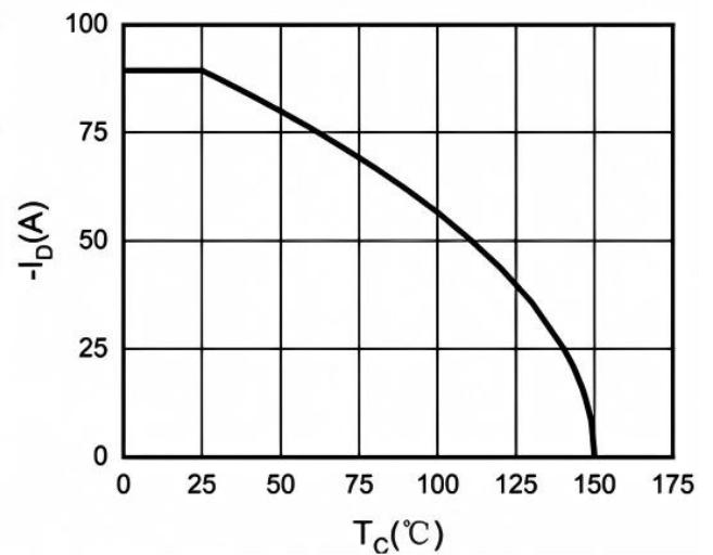
Fig.4 Drain Current
