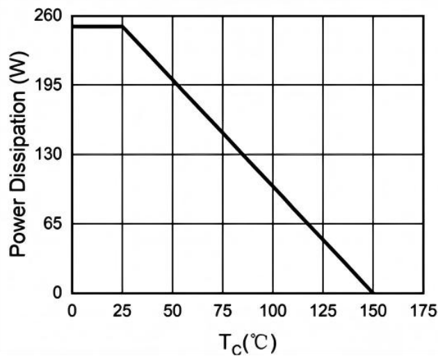
Fig.3 Power Dissipation
