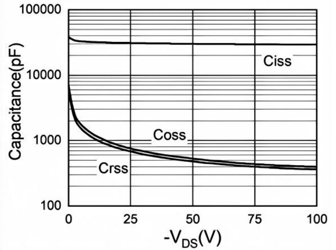
Fig.8 Capacitance
