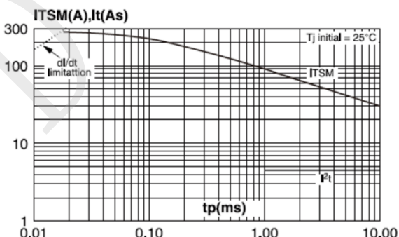
Fig. 9: Non-repetitive surge peak on-state current for a sinusoidal pulse with width t_p < 10\text{ ms} , and corresponding value of I^2t .
