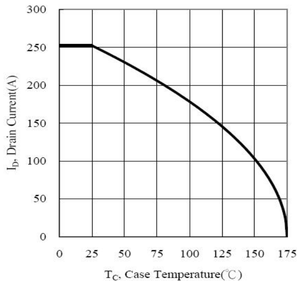
2. Drain Current
