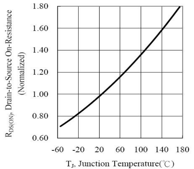
6. Drain-to-Source On-Resistance
