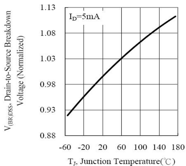
4. Drain-to-Source Breakdown Voltage
