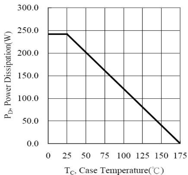
1. Power Dissipation
