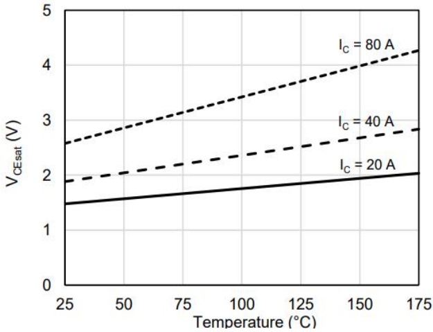
Fig.7 Vcesat vs. Junction Temperature
