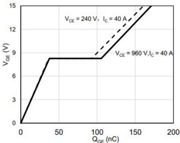
Fig.5 Gate charge
