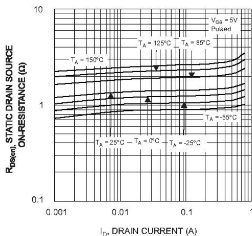
Fig. 5 Static Drain-Source On-Resistance vs. Drain Current
