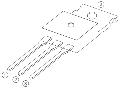
TO-220C
