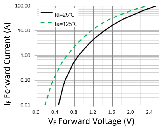
Figure 1. Forward Characteristic(typ.)
