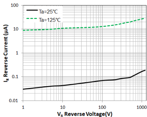
Figure 2. Reverse Characteristic(typ.)
