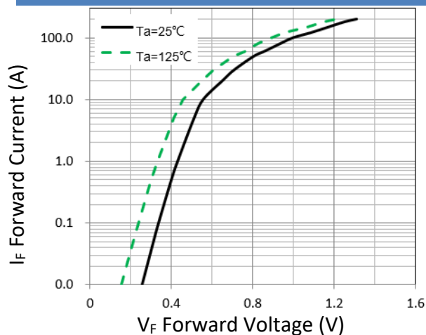
Figure 1. Forward Characteristic(typ.)
