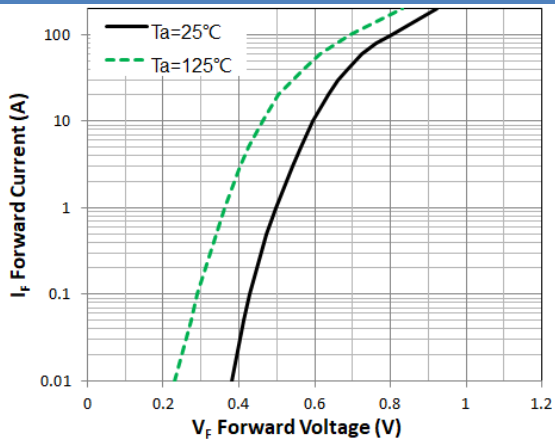
Figure 1. Forward Characteristic(typ.)
