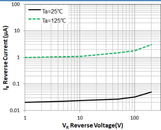
Figure 2. Reverse Characteristic(typ.)
